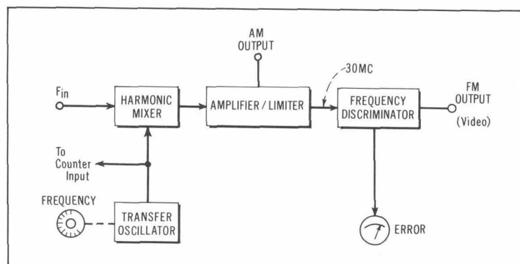
Fig. 7. Block diagram of Microwave Frequency Converter operating in FM mode.
