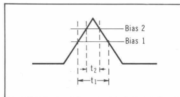
Fig. 9. Drawing showing how changing bias on sampling diodes changes sample width, hence, bandwidth of sampling circuit.
