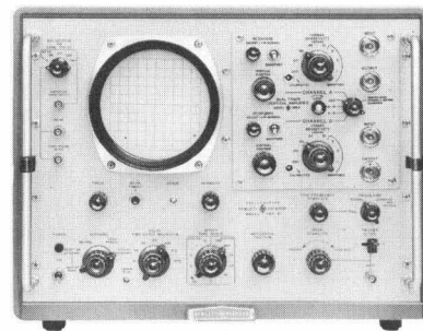
Fig. 5. Model 188A plug-in unit installed in 185A Sampling Oscilloscope.
