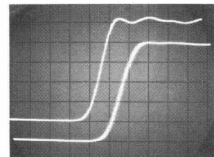
Fig. 10. Oscilloscope showing typical effect of setting "Response Adjust" control. Lower trace (70 psec rise time) shows typical "Normal" response. Upper trace (50 psec rise time) shows "Response Adjust" control set for fastest rise time which increases bandwidth but reduces sensitivity to random signals.
