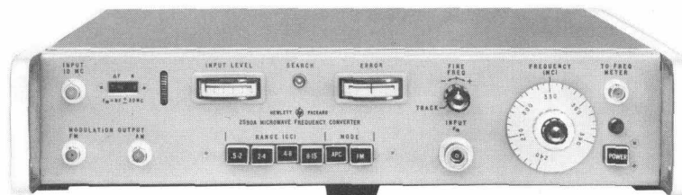
Fig. 5. Hewlett-Packard Model 2590A Microwave Frequency Converter enables accurate counter measurements of microwave frequencies in 0.5 to 15 Gc range. Built-in roll-chart (upper left) simplifies determination of frequency. Converter also has AM and FM demodulators to provide additional information about measured signals. Transfer oscillator may be used independently as 240-390 Mc signal source.
