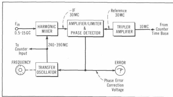
Fig. 4. Skeleton block diagram of -hp- 2590A Microwave Frequency Converter in automatic phase control (APC) mode of operation. Automatic phase control locks transfer oscillator to sub-multiple of input frequency for accurate frequency measurement.
