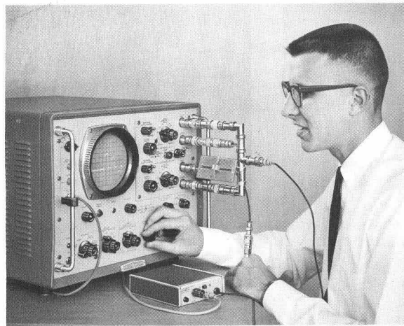
Fig. 1. New Model 188A dual-channel plug-in for -hp- Sampling Oscilloscope permits viewing signals of 90 picoseconds rise time, i.e., to above 4 gigacycles in frequency (to 8 Gc at reduced sensitivity). Plug-in is designed to view signals on 50-ohm lines by bridging line so that measured circuit is not disrupted.
