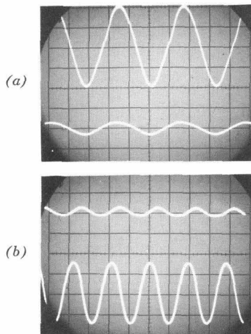
Fig. 3. Scope photos show additional information available from -hp- Model 2590A Microwave Frequency Converter. Incidental AM on an FM signal is shown as lower trace in (a) while upper trace shows demodulated FM. Lower trace in (b) shows envelope of AM signal while upper trace shows incidental FM on same signal.
